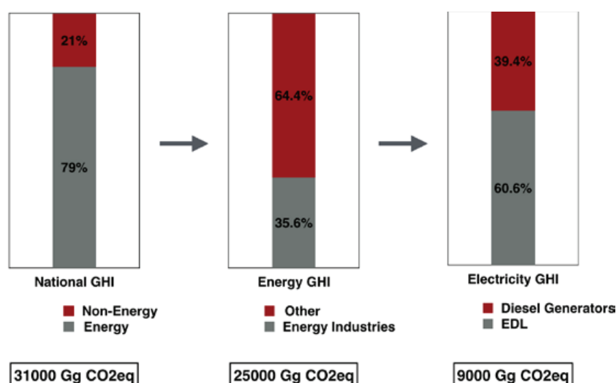
Figure 27: Estimated national, energy sector and electricity sector GHI in 2018
