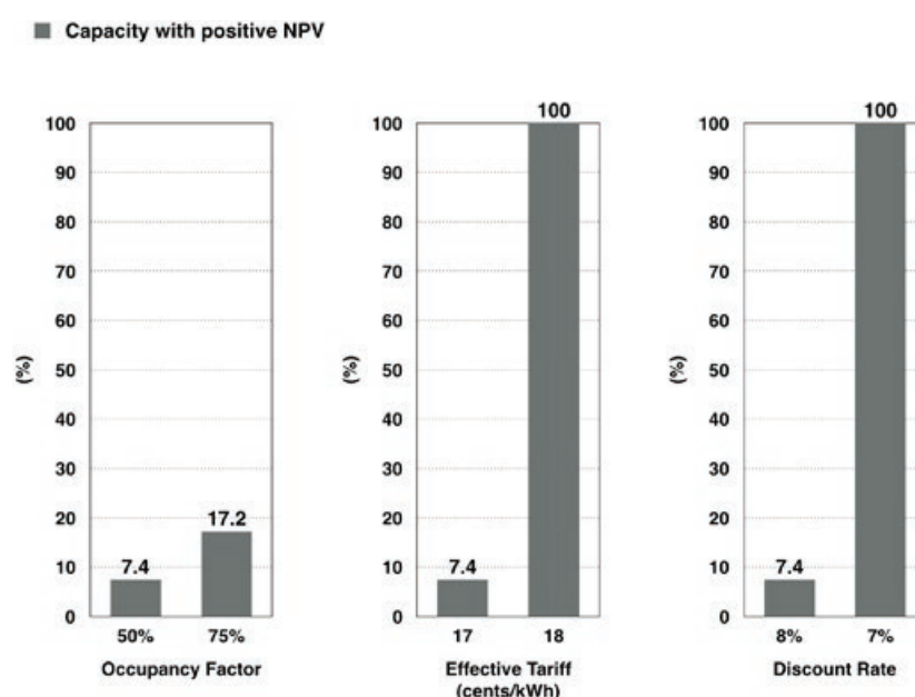
Figure 21: Percentage of on-grid rooftop solar PV capacity of projects with a positive NPV as a function of occupancy factor, effective tariff and discount rate
